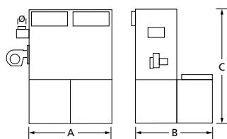
UNIT-HP 300
